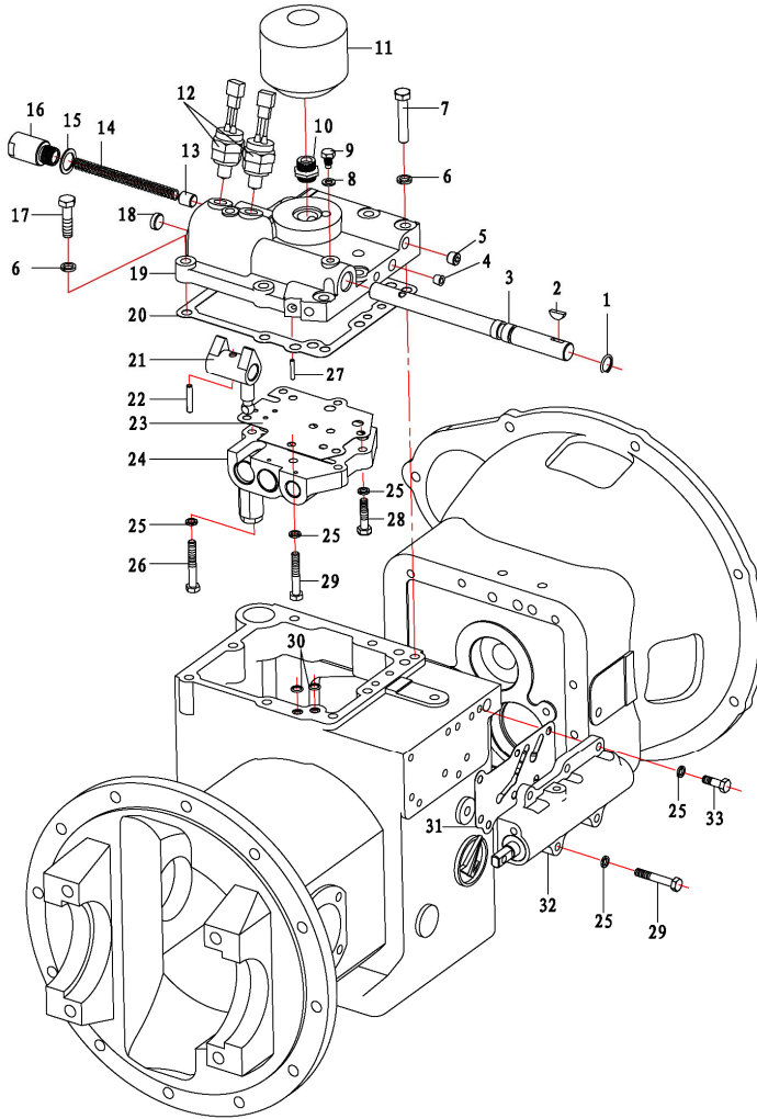
Fig.19 Cover control valve & inching valve (tor-con type)
