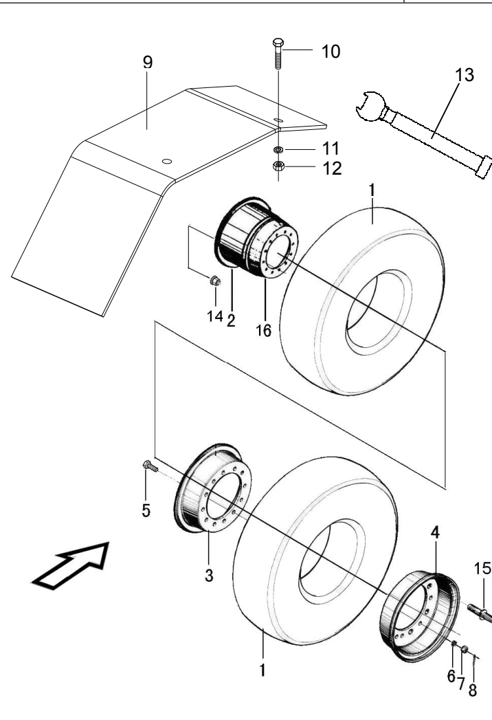
图 5 1.0t-1.8t 前轮 (双轮) Fig.5 1.0t-1.8t Front wheel (Double tyre)
