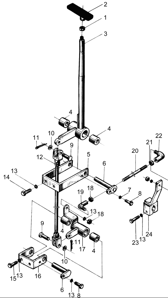
Fig.7 Change over control assy
