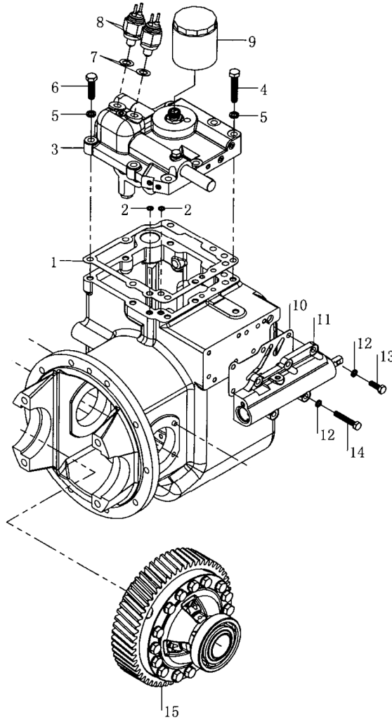
Fig.12 Cover control valve & inching valve (tor-con type) SHAOXING
