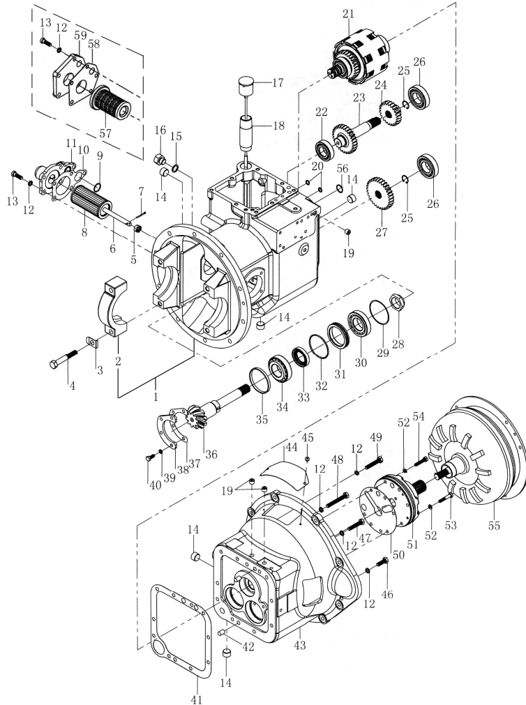
Fig.10 Transmission(tor-con type)
