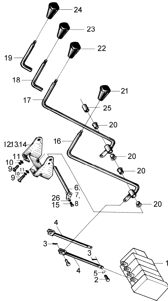
图7 多路阀操纵 Fig.7 Multi-way valve control
