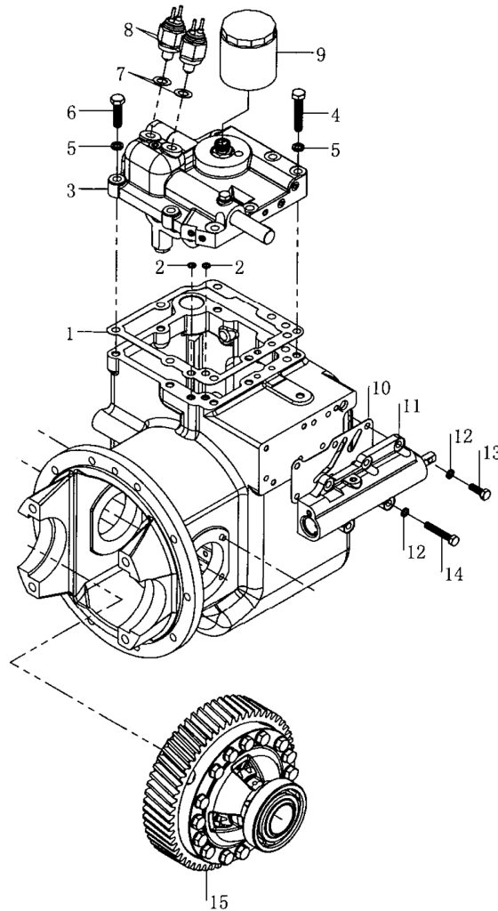
图 12 盖、控制阀、微动阀（液力式）绍兴 Fig.12 Cover control valve & inching valve (tor-con type) SHAOXING
