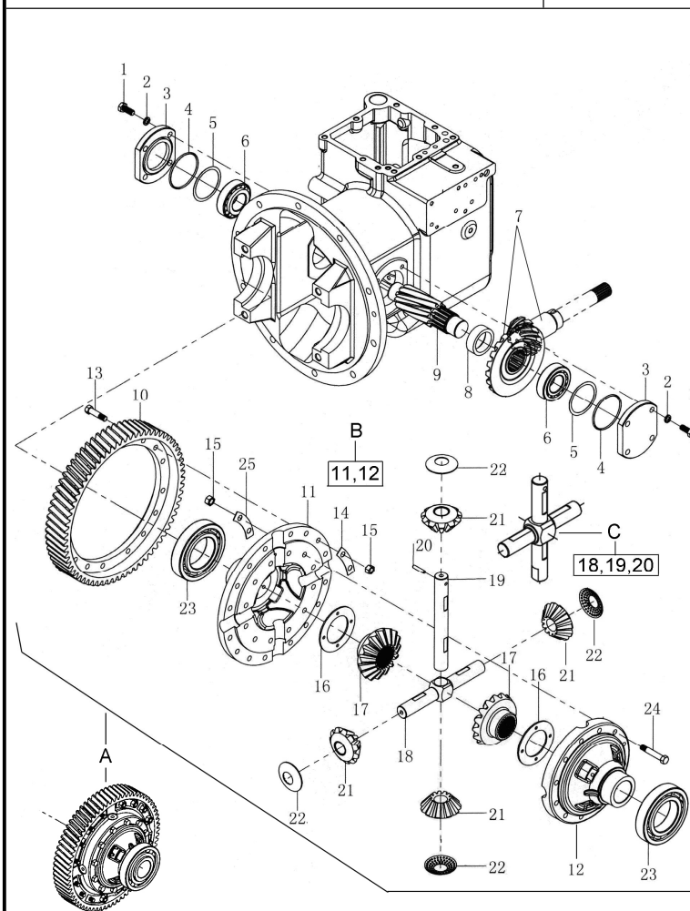
图 13 减速器和差速器 (绍兴) Fig.13 Reduction & differential (ShaoXing)
