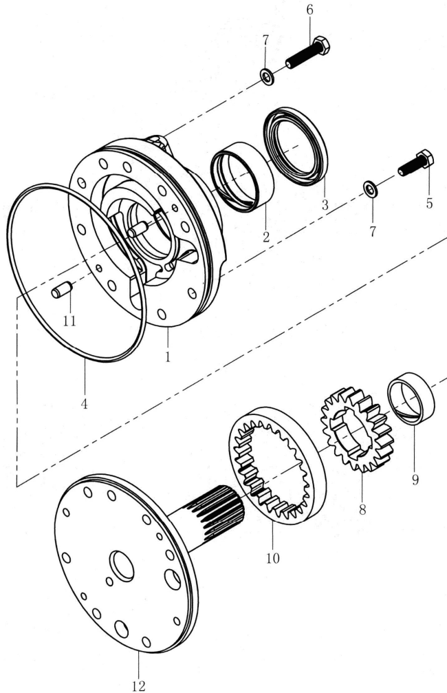
图 14 供油泵（液力式）绍兴 SHAOXING Fig.14 Charging pump(tor-con type)
