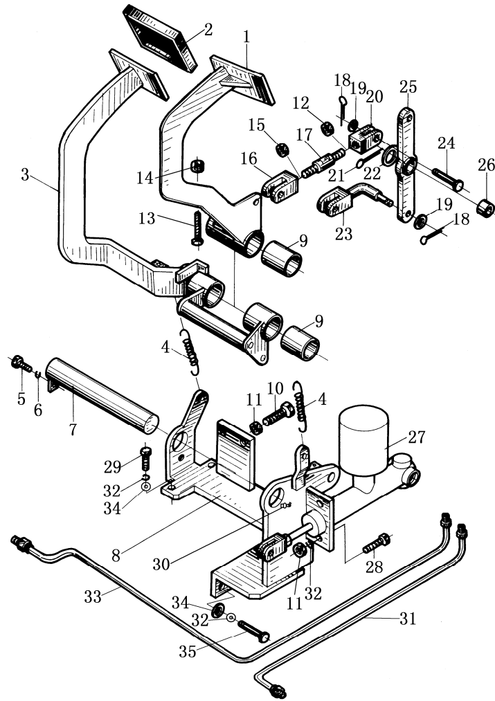
图2 制动微动操纵总成&制动油管总成 Fig.2 Brake and inching control assy & Brake pipe assy
