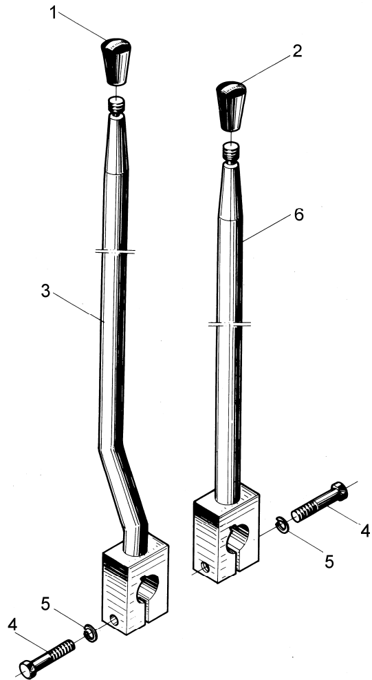
图6 换档操纵总成 Fig.6 Change over control assy
