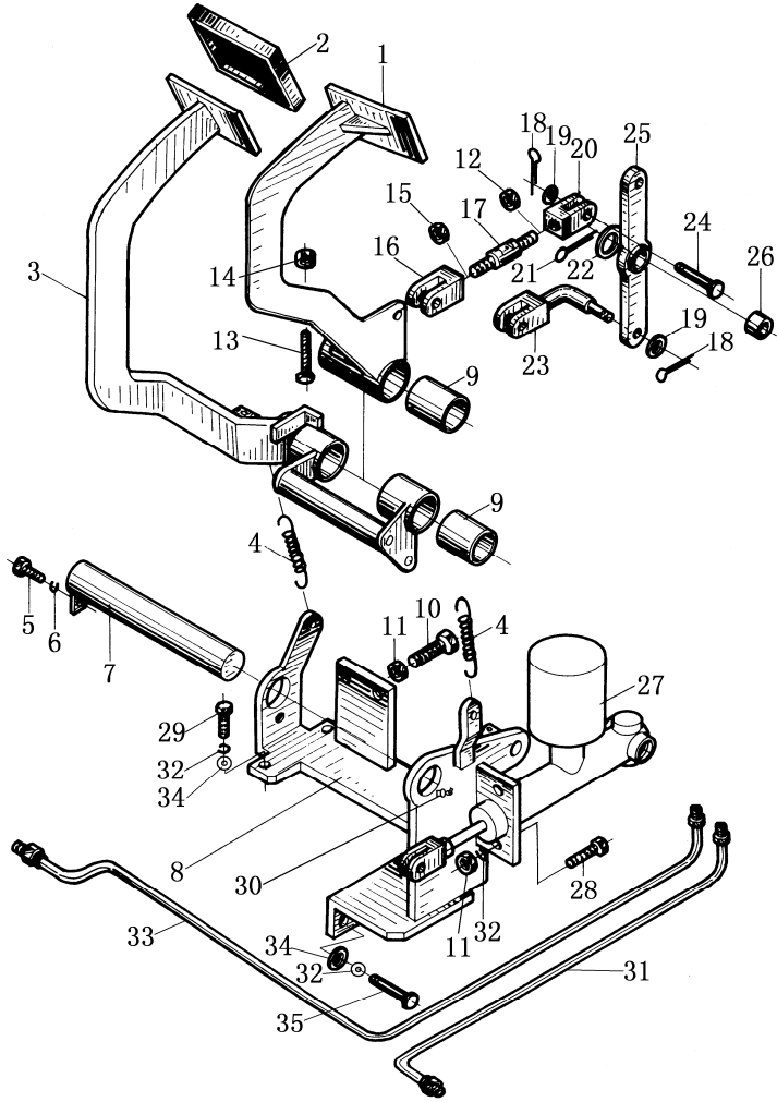
Fig.2 Brake and inching control assy & Brake pipe assy
